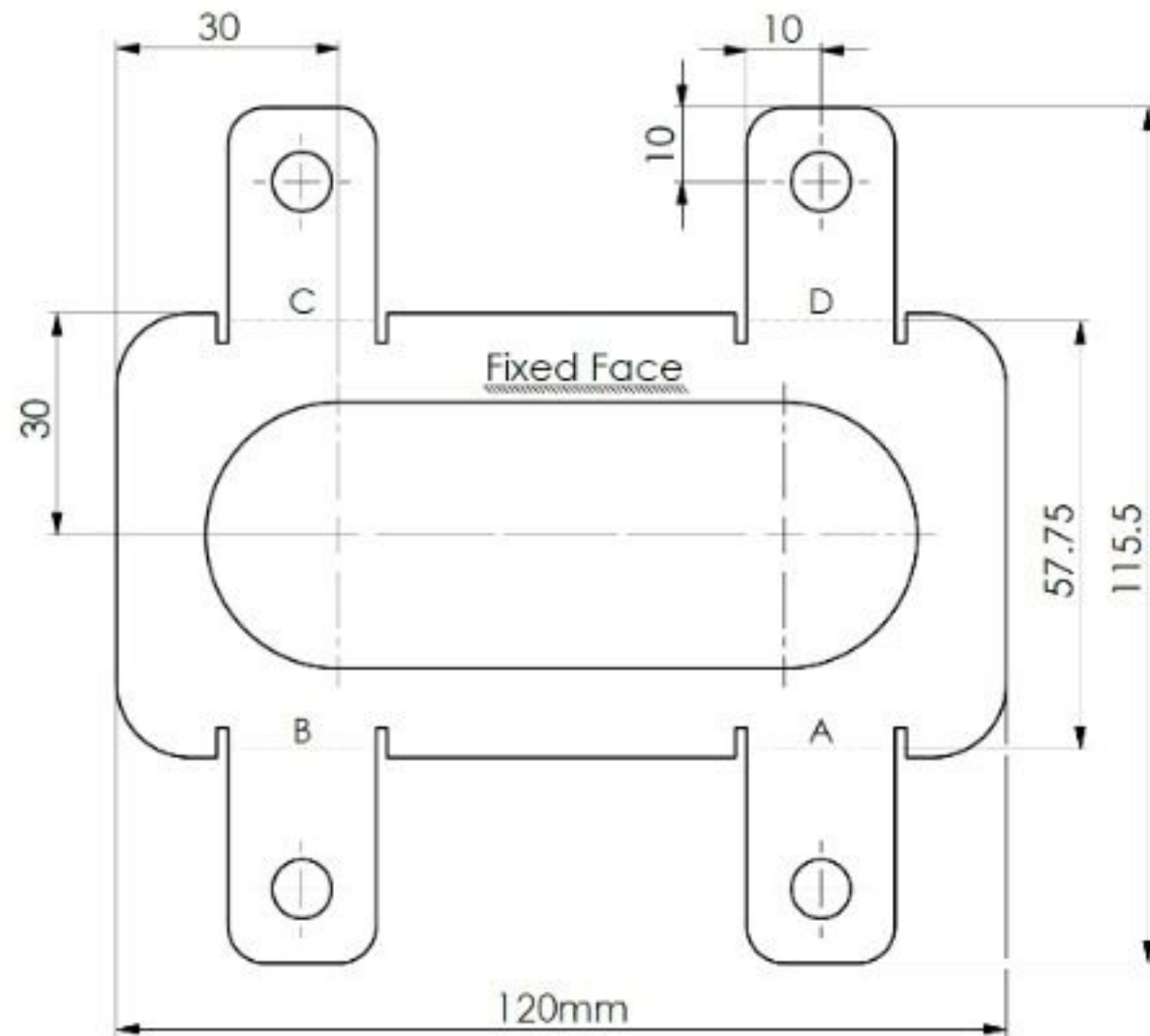
FLATTEN VIEW SCALE 1:1
