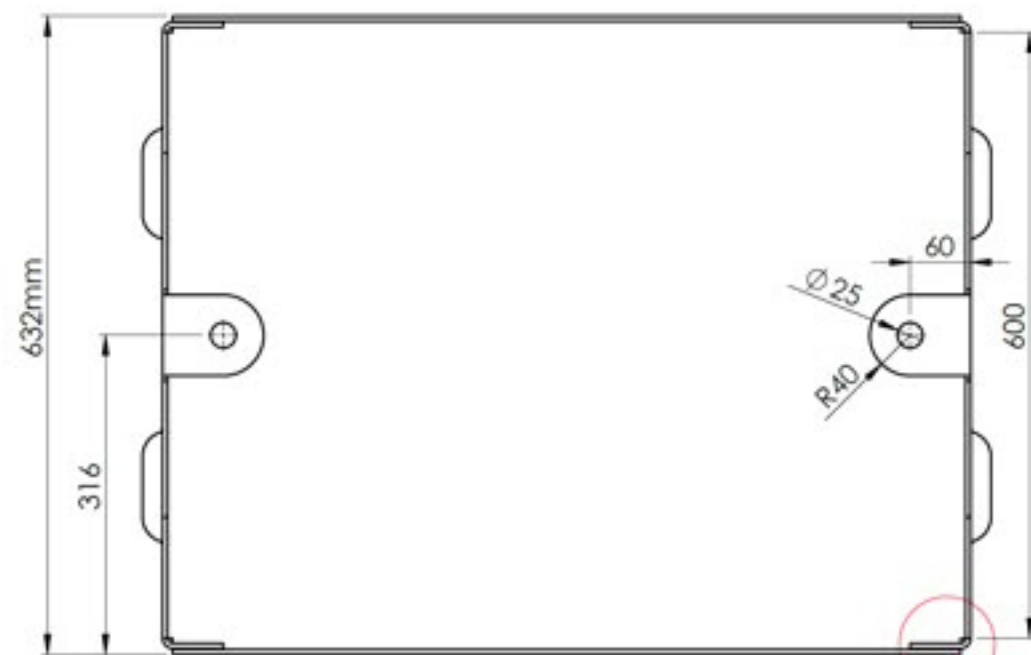
TOP VIEW
