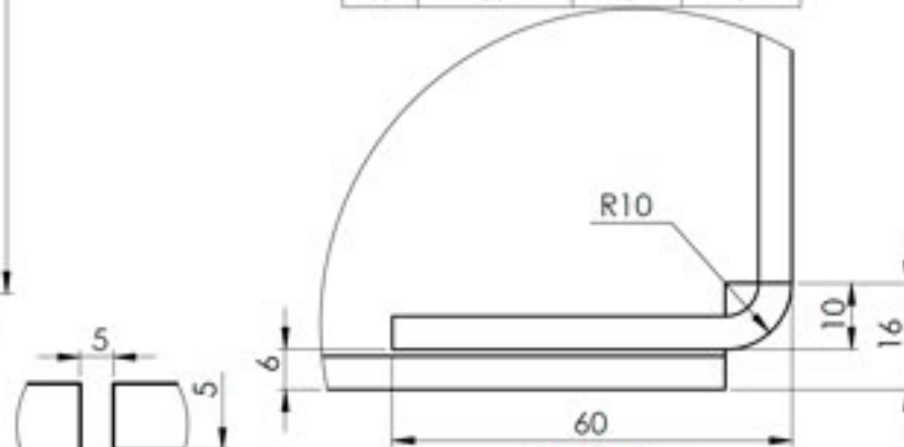
DETAIL H SCALE 1 : 1
