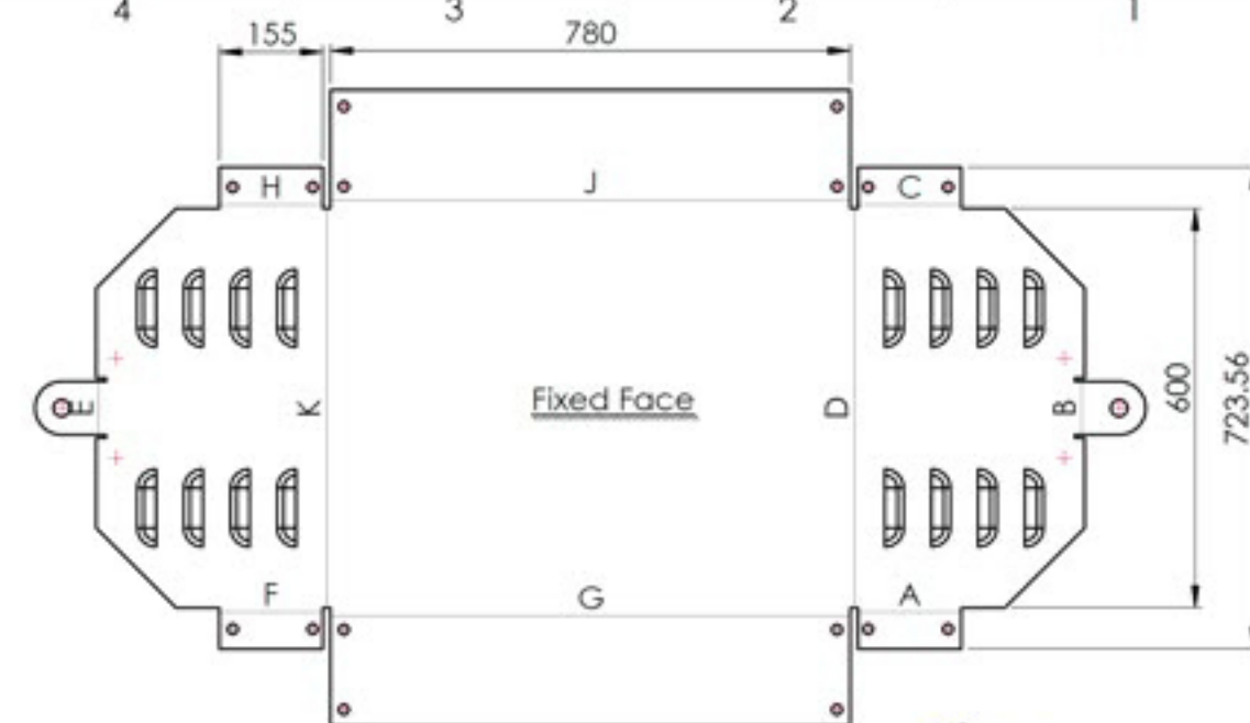
FLAT PATTERN
