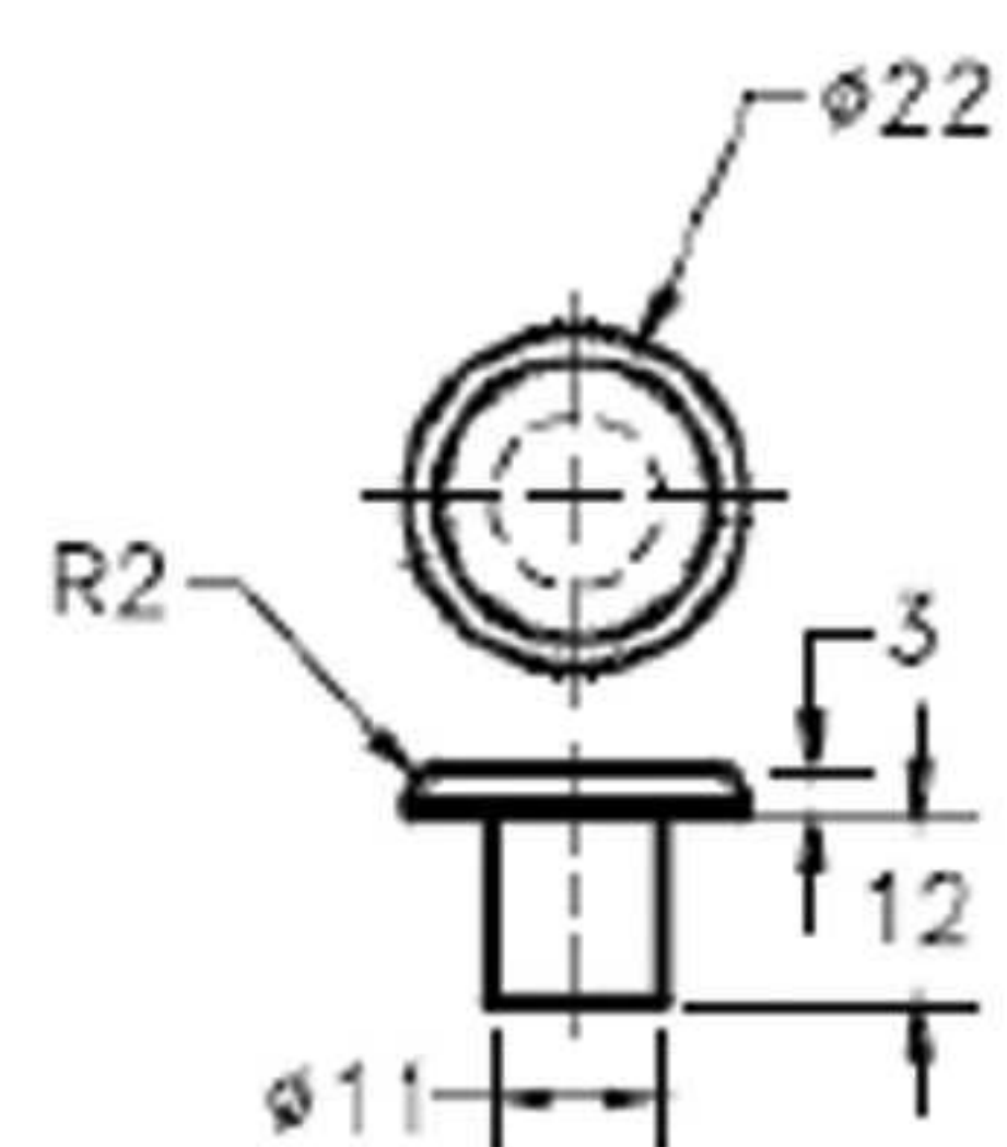
Piston Pin Plug
