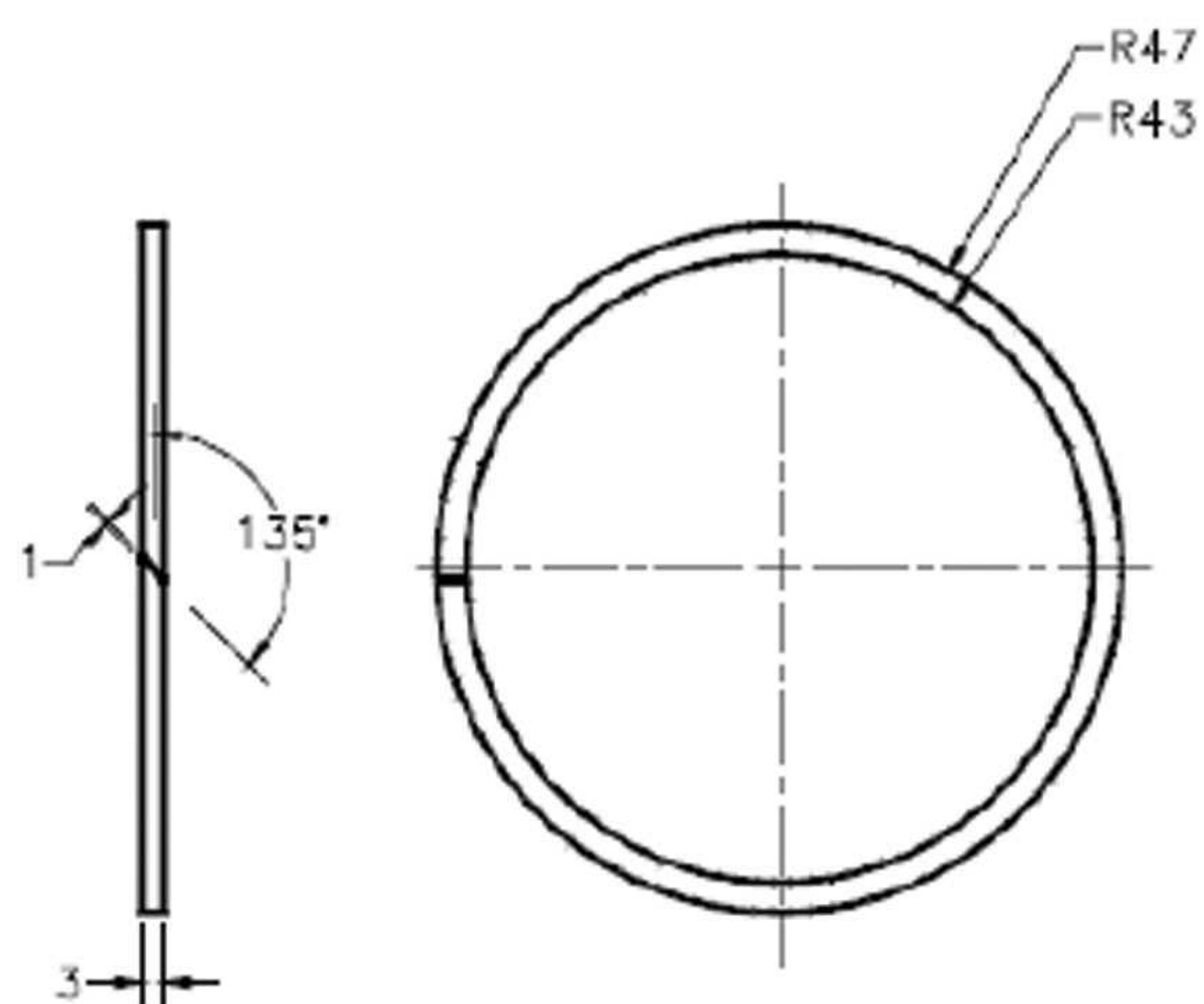
Piston Rings
