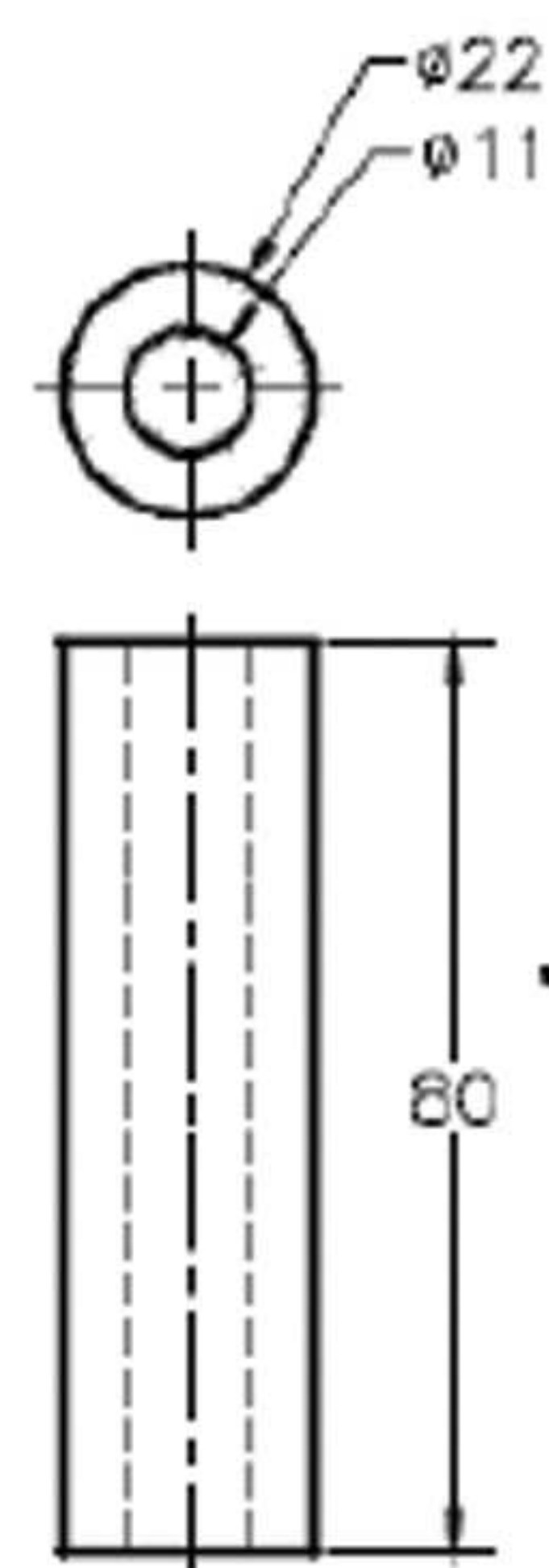
Piston Pin
